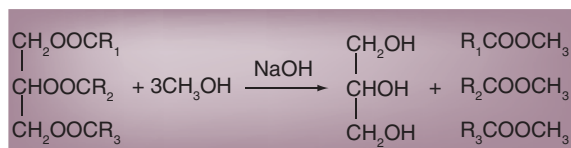
Figure 2. Base transesterification to biodiesel.
